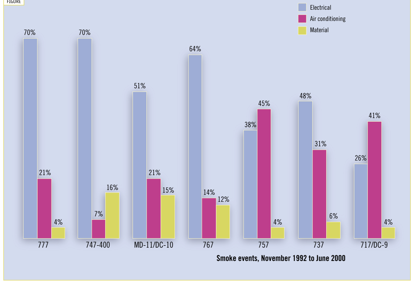
1 SUMMARY PROFILE OF REPORTED SMOKE EVENTS IN PRESSURIZED AREAS OF THE AIRPLANE
